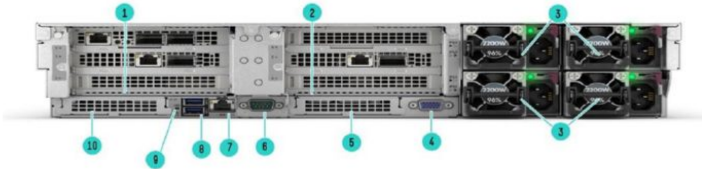
HPE ProLiant Compute DL384 Gen12 - Rear View
